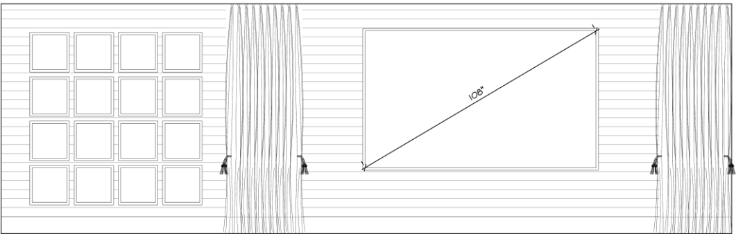
Screen Wall Elevation
